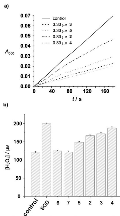
Figure 4. a) Kinetics of the reduction of ferricytochrome c (550 nm) without and with the fullerenes at room temperature. b) Production of H_2O_2 by SOD (25 \mu M ) and fullerenes (25 \mu M ) from KO_2 (500 \mu M ; pH 7.8; 37 °C).
