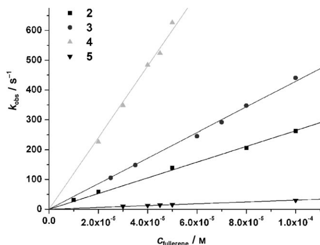
Figure 3. k_{obs} as a function of fullerene concentration for the reaction between fullerenes and saturated KO_2 in DMSO solution at room temperature.
